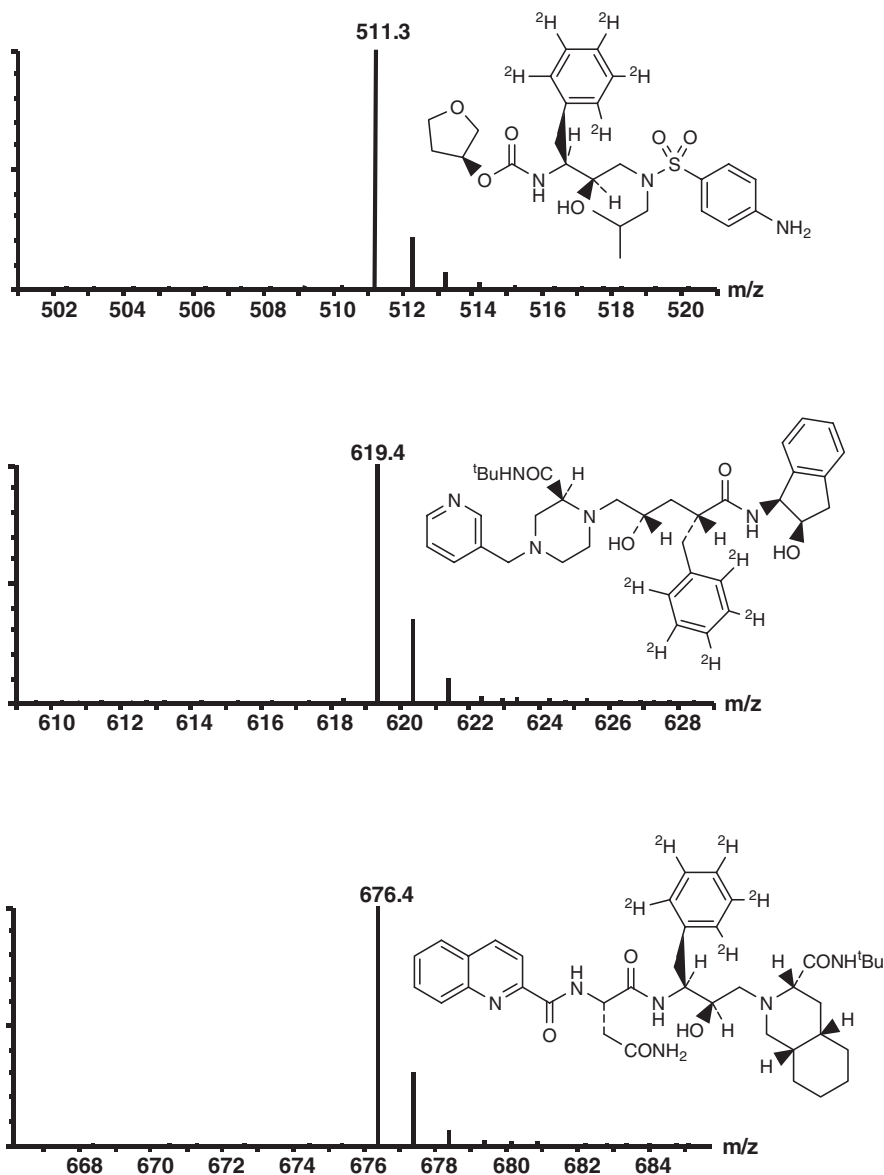
Figure 3. MS TOF ESI (+) of [ 2 H 5 ]-PIs
